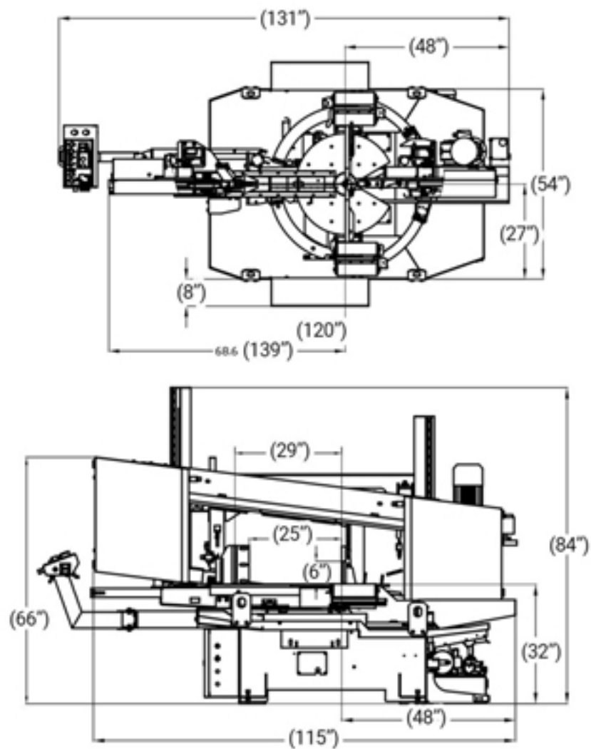
Dimensional Drawings of DCDS-600SA
